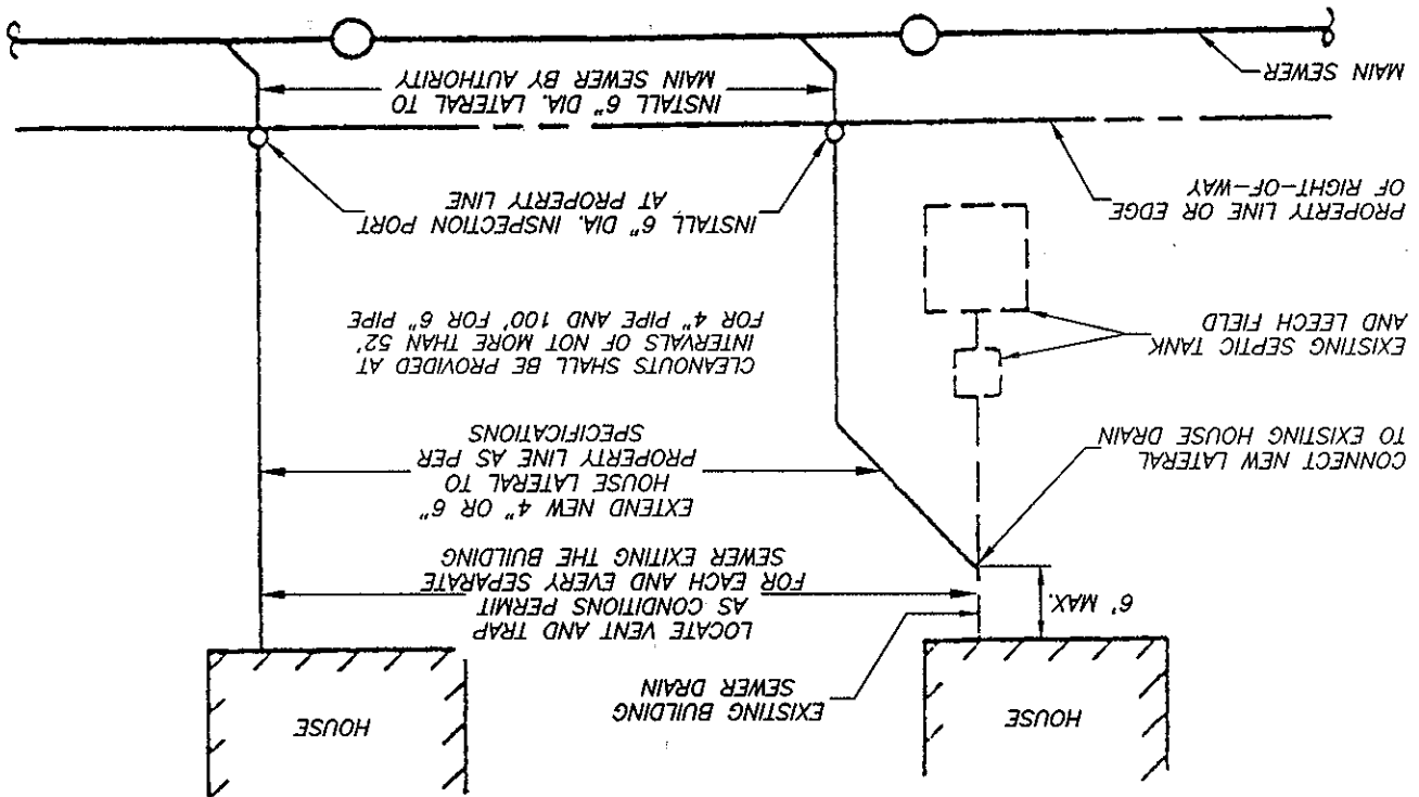
SEPTIC TANK BYPASS PLAN
